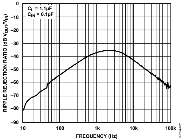
Figure 21. ADR3550 Ripple Rejection Ratio vs. Frequency
